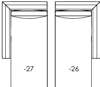
XXXX-27 LAF Chaise | XXXX-26 RAF Chaise w37.5 d71 h32.5 in. ah26 sh19.5 sd53 iw30 in. Standard with (1) 18" throw pillow
