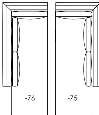
XXXX-76 LAF Cuddle Chaise w37.5 d94.5 h32.5 in. ah26 sh19.5 sd78 iw21.5 in. XXXX-75 RAF Cuddle Chaise w37.5 d94.5 h32.5 in. ah26 sh19.5 sd78 iw21.5 in. Standard with (1) 18" throw pillow
