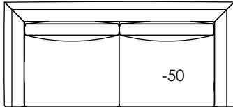
XXXX-50 Sofa w83 d37.5 h32.5 in. ah26 sh19.5 sd21.5 iw68 in. Standard with (2) 18" throw pillows
