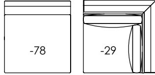
XXXX-78 Armless Chair w34 d37.5 h32.5 in. ah26 sh19.5 sd21.5 iw34 in. XXXX-29 Corner Chair w34 d37.5 h32.5 in. ah26 sh19.5 sd21.5 iw21.5 in.
